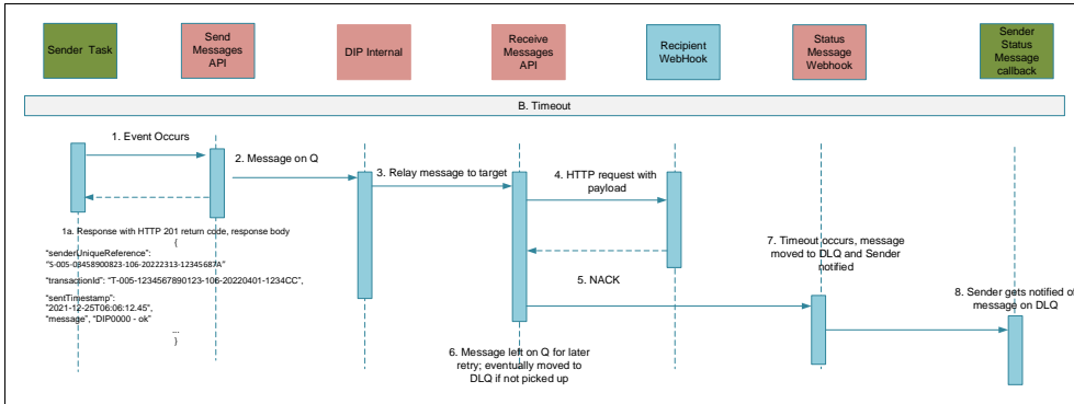
Figure 12 – Recipient Timeout
